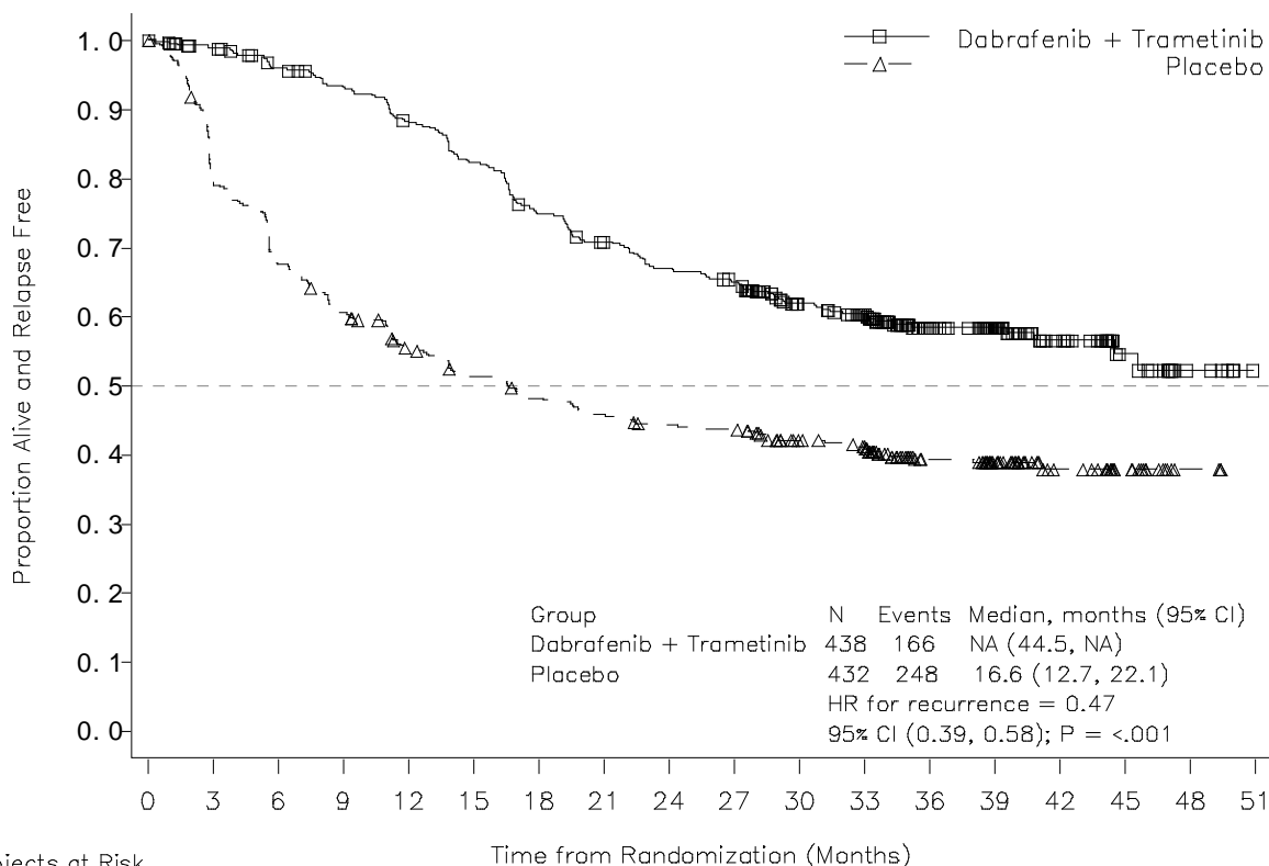
Figure 12-5 COMBI-AD - Relapse-free survival Kaplan-Meier curves (ITT population)
